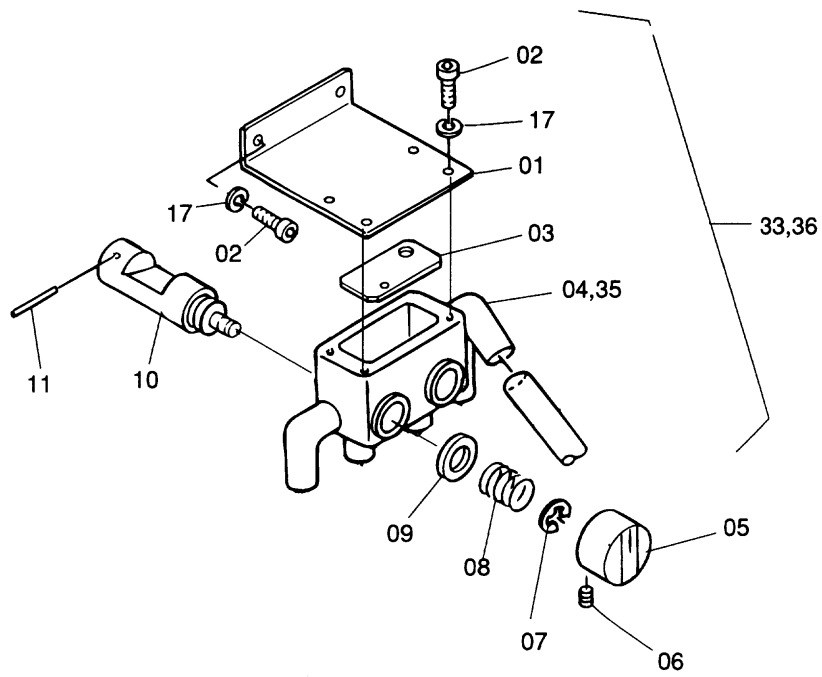
Control Valve ( OP-S )
