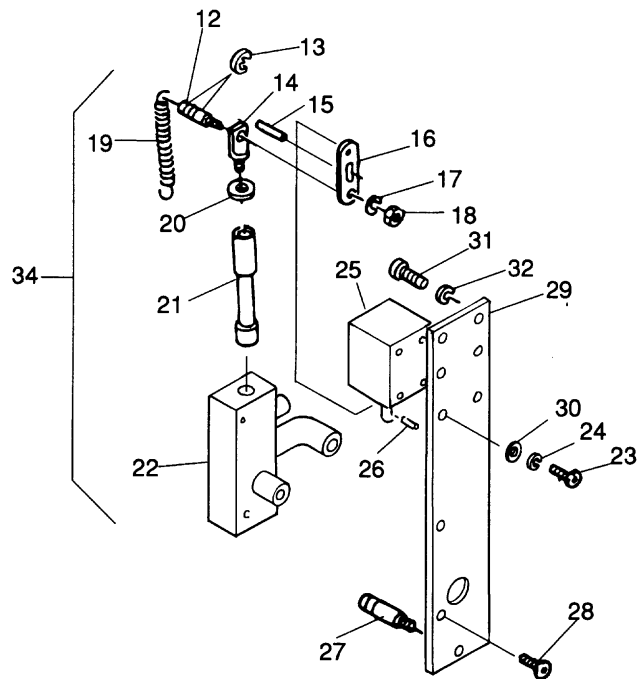
Blanket-Cleaner Valve
